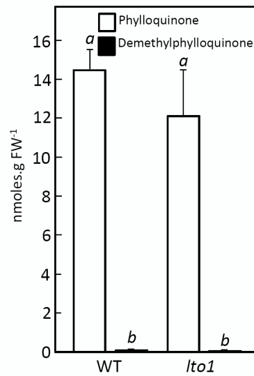
Supplemental Fig.1. Quantification of phyloquinone and of demethylphyloquinone in the leaves of wild-type and lto1 knockout plants. Same letter annotations above the error bars indicate that the corresponding values are not significantly different as determined by Fisher's least significant difference test from ANOVA ( p > 0.1 ). Data are the means of 4 replicates \pm SE.
