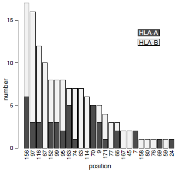
Fig. S1 The distribution of HLA pairs with a single substitution ( n=138 ). The positions are ranked according to their frequencies among the HLA pairs.
