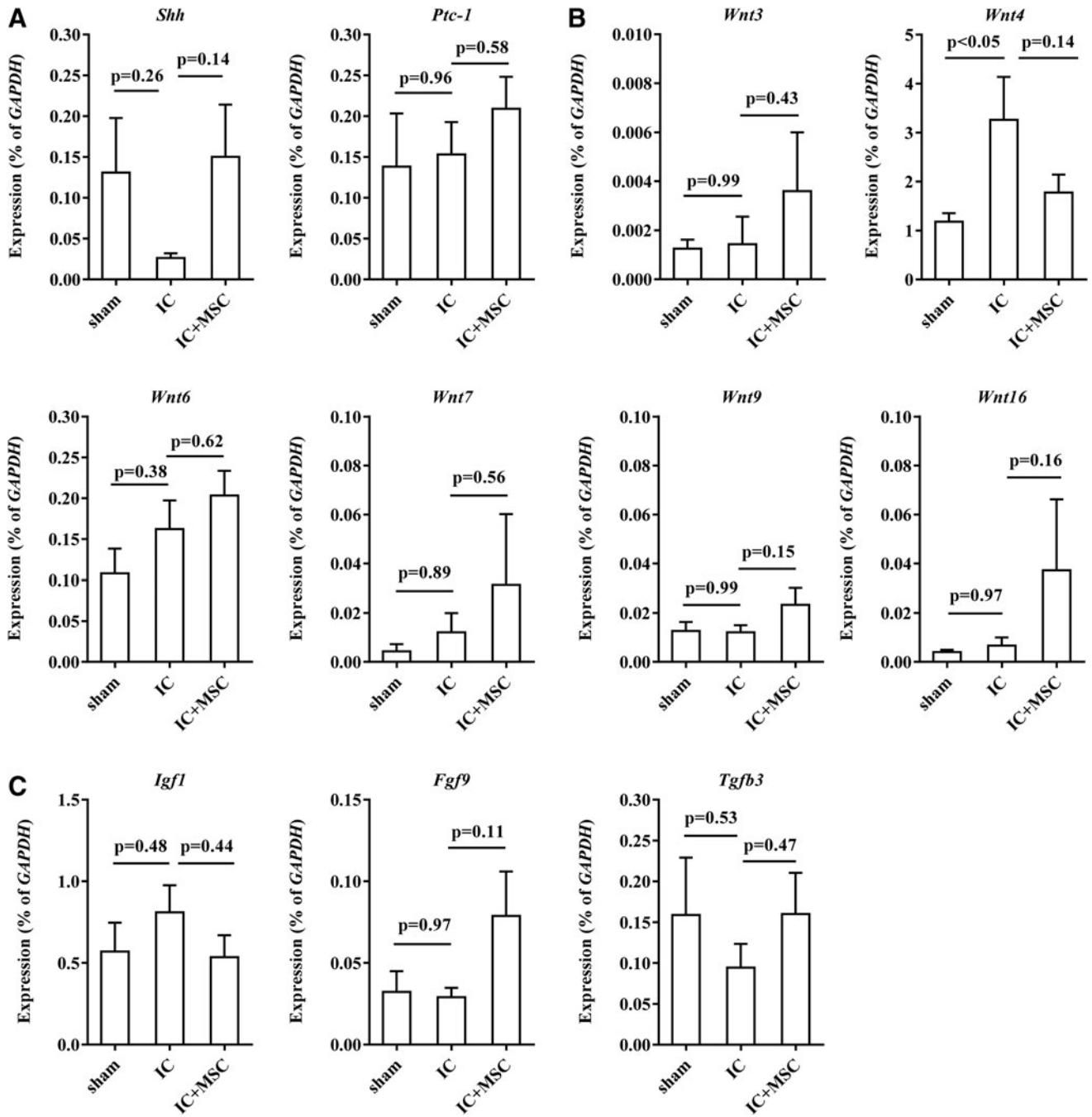
SUPPLEMENTARY FIG. S3. RQ-PCR analysis of (A) Shh , (B) Wnt , and (C) downstream growth factors in the indicated bladder tissues. The expression level is represented as % Gapdh (as determined using five or more independent experiments) and is shown as the mean \pm SEM ( P < 0.05 in comparison with IC group bladders, one-way ANOVA with Bonferroni post-test).
