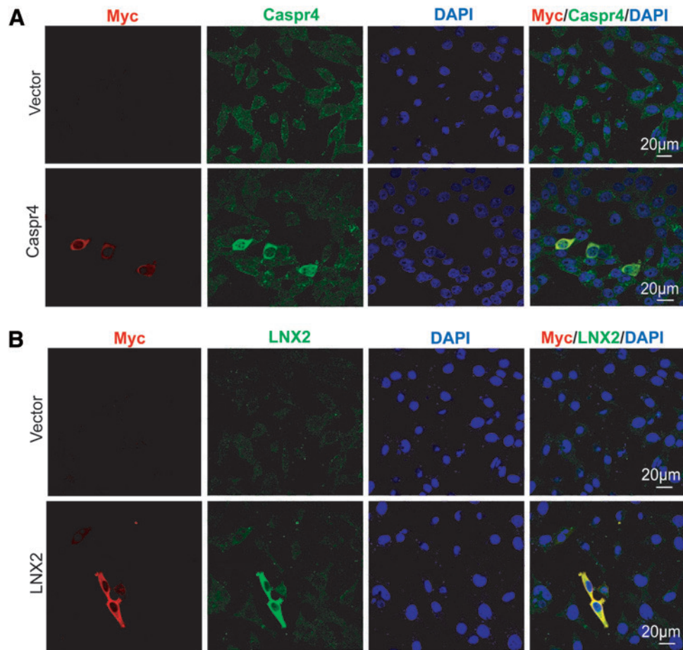
SUPPLEMENTARY FIG. S4. Validation of antibodies against Caspr4 and LNX2. HEK293 cells transfected with Caspr4-myc ( A ) or LNX2-myc ( B ) or an empty vector as the control were stained for myc and Caspr4 ( A ) or LNX2 ( B ). Caspr4 and LNX2 immunoreactivity were detected in Caspr4-myc- and LNX2-myc-transfected cells and colocalized with myc, respectively. Scale bars: 20 \mu m.
