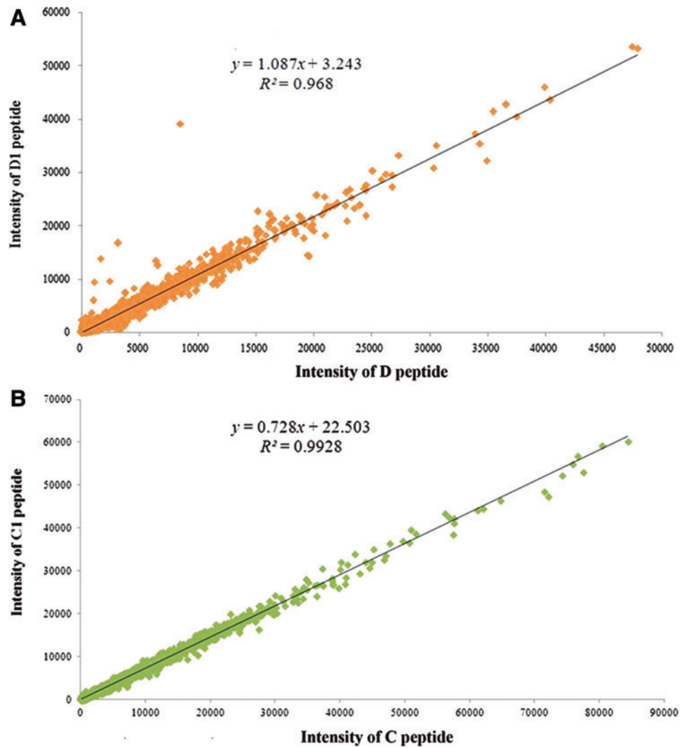
SUPPLEMENTARY FIG. S1. Correlation between peptide label intensities with different iTRAQ tags. (A) D and D1 indicate 115 and 116, respectively. (B) C and C1 indicate 119 and 121, respectively.
