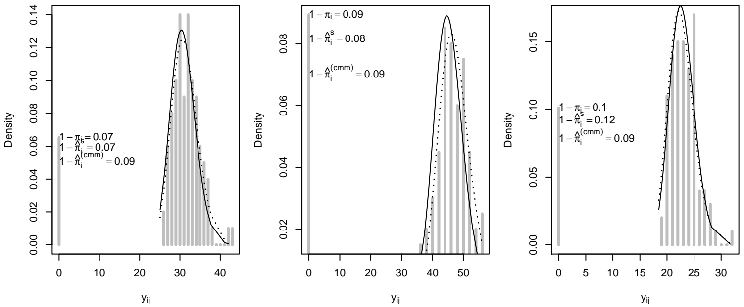
Supplementary Figure 1. Model misspecification. Here Y_{ij} is simulated from a log-normal (LNN) distribution. Solid lines are the true density function and dotted lines are the CMM fitted density function.
