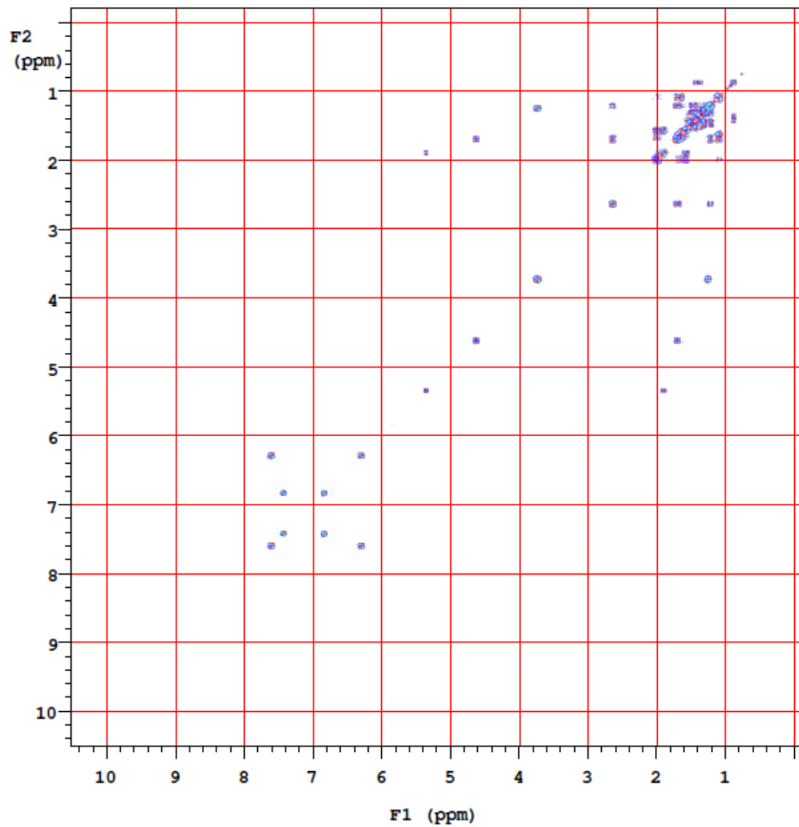
Figure S3E. COSY NMR spectrum of oleanolic aldehyde coumarate in CDCl 3 (400 MHz)
