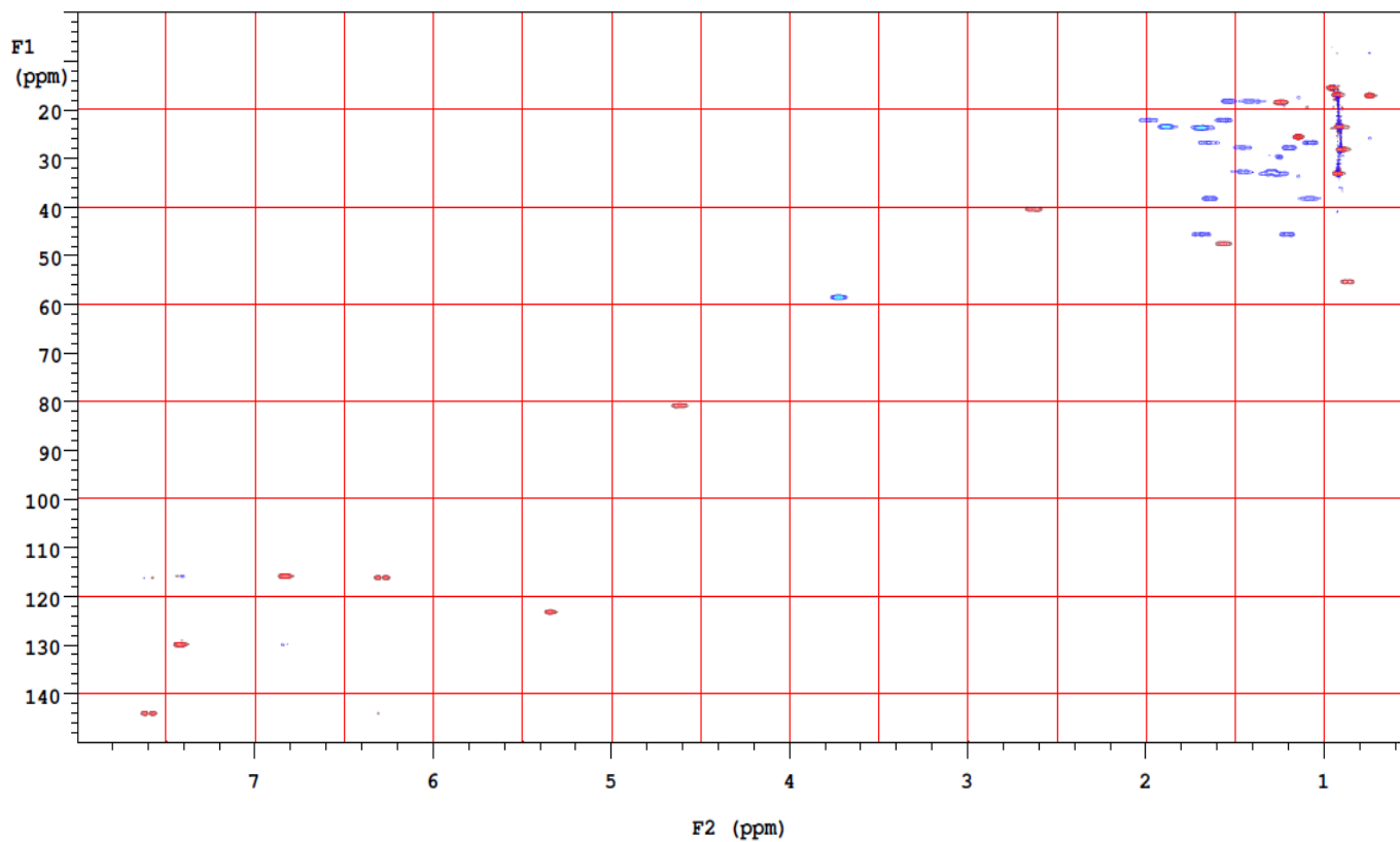
Figure S3D. HMBC NMR spectrum of oleanolic aldehyde coumarate in CDCl 3 (400 MHz)
