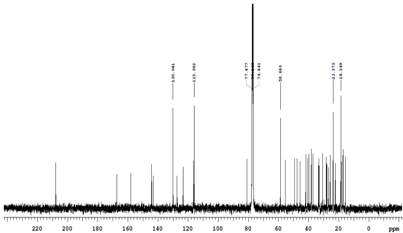
Figure S3B. ^{13}\text{C} NMR spectrum of oleanolic aldehyde coumarate in \text{CDCl}_3 (400 MHz)
