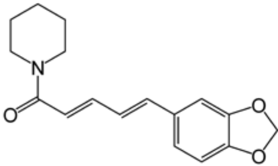
Figure 1 Piperine molecular structure
