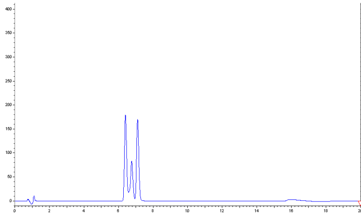
(B) Piperine split peak when processed after 6 hours in red light
