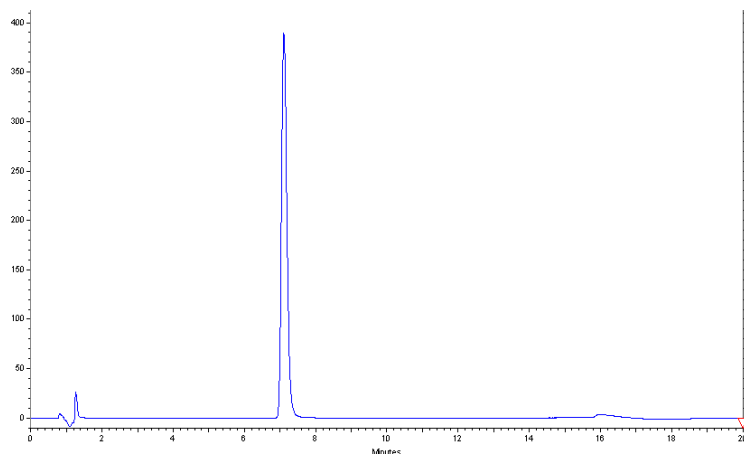
(C) Piperine single peak when processed in minimal ambient light
