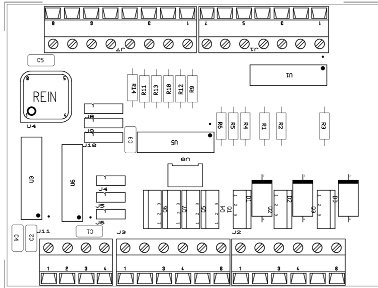
Main board component side
