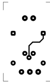
Photo emitter component side
