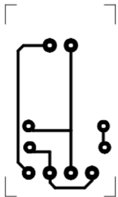
Photo receiver solder side
