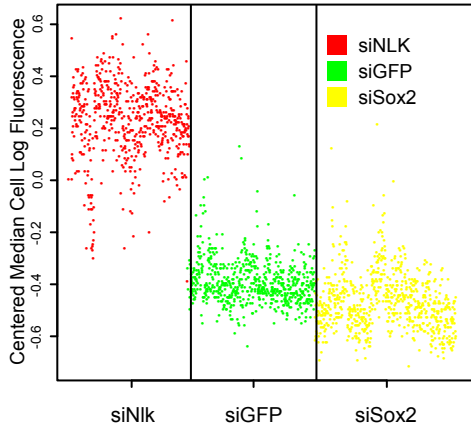
True Clustering
