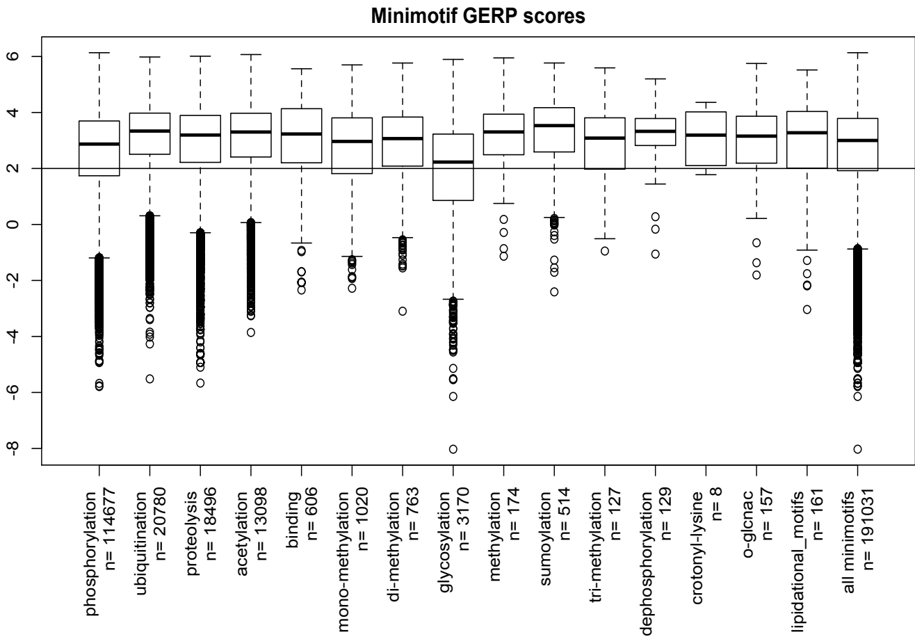
Figure S3. Quartile plots of GERP scores for different types of minimotif subactivities.
