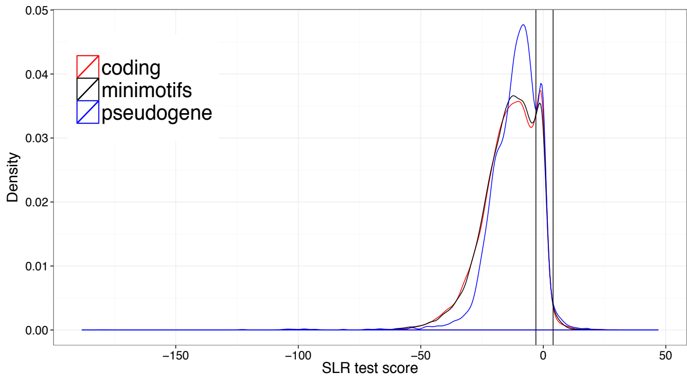
Figure S2. Density plot of SLR scores for different genomic regions. Vertical lines indicated threshold for negative, neutral, and positive selection.
