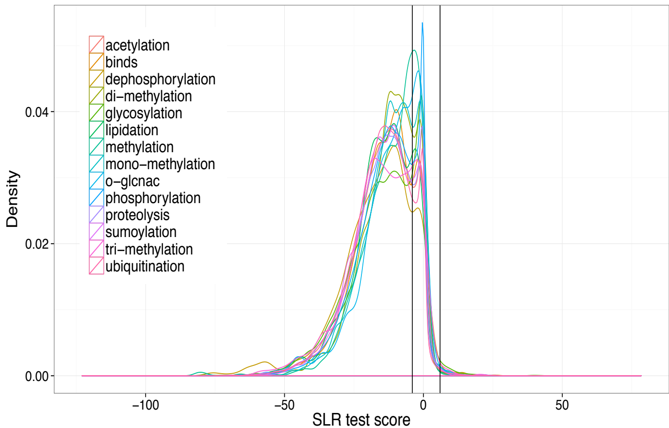
Figure S4. Density plot of SLR scores for different minimotif subactivities. Vertical lines indicated threshold for negative, neutral, and positive selection determined from Fig. S2 .
