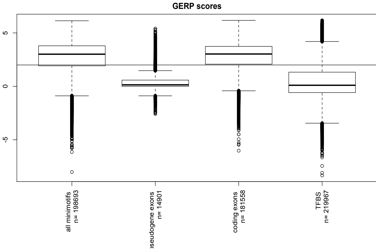
Figure S1. Quartile plots of GERP scores for different genomic regions.
