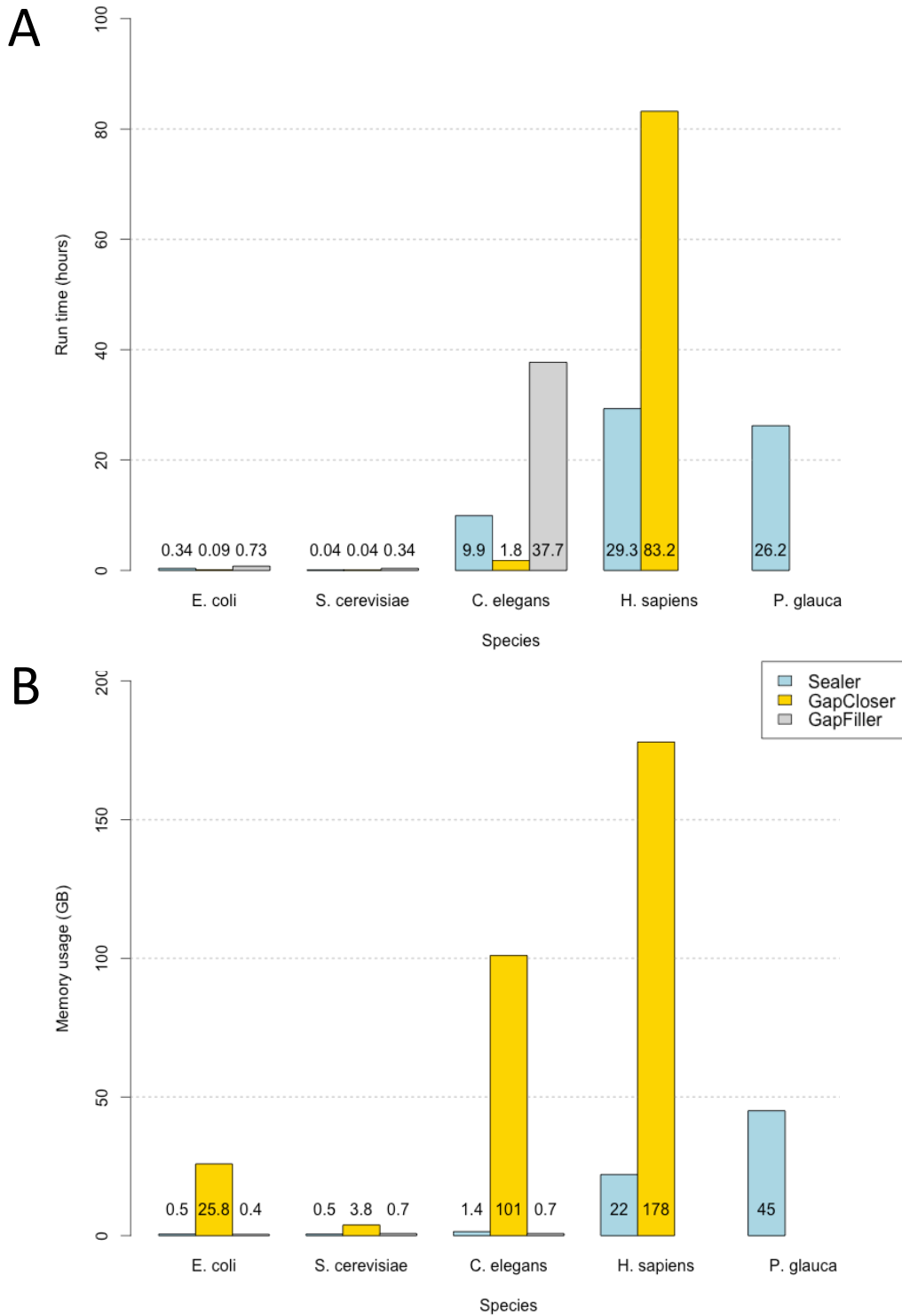
Supplemental figure S2. Compute resource required by Sealer, GapCloser and GapFiller for closing gaps in the E.coli K12, S. cerevisiae , C. elegans , H. sapiens and P. glauca draft genome assemblies. A) Run time B) Memory usage.
