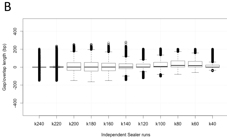
Supplemental figure S3. Individual Sealer H. sapiens runs at unique values of -k and -P . A) Gap closing yield as a function of k and varying with the maximum number of path allowed. B) gap size distribution for individual Sealer runs at unique values of k .
