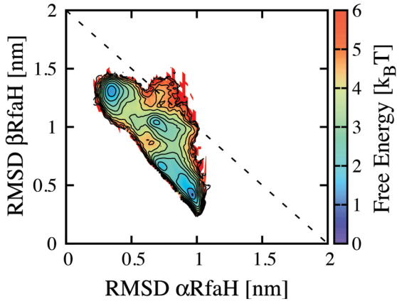
mixed dihedrals
