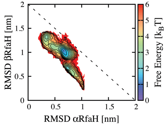
dual-basin dihedrals
