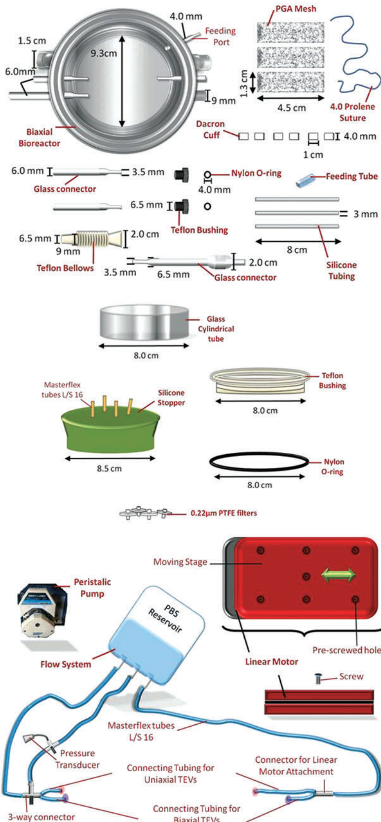
SUPPLEMENTARY FIG. S1. List of all individual parts of the biaxial bioreactor system.
