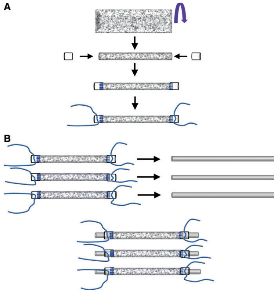
SUPPLEMENTARY FIG. S2. Tubular polyglycolic acid (PGA) scaffold fabrication. (A) Construction of tubular PGA scaffolds with Dacron cuffs at the two ends using a 4.0 Prolene suture. (B) Insertion of silicone tubing inserted into lumens of PGA scaffolds.
