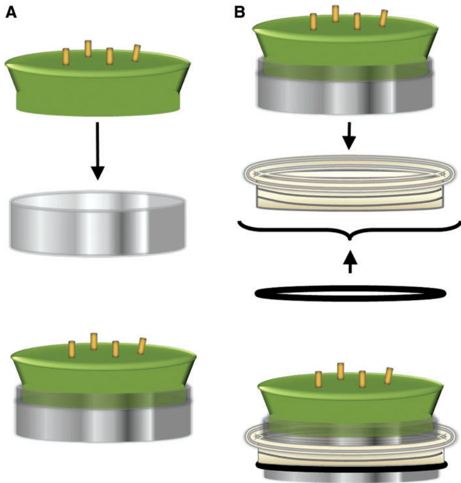
SUPPLEMENTARY FIG. S3. Bioreactor cap assembly. (A) A silicone stopper with tubing for air filters is inserted into a glass cylinder. (B) The whole unit is fitted into a Teflon bushing and an O-ring is pulled over the glass cylinder from the bottom .
