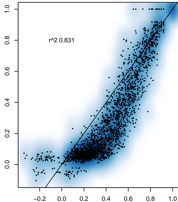
30% missing data
