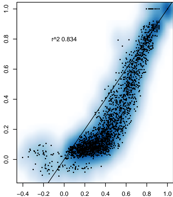
20% missing data
