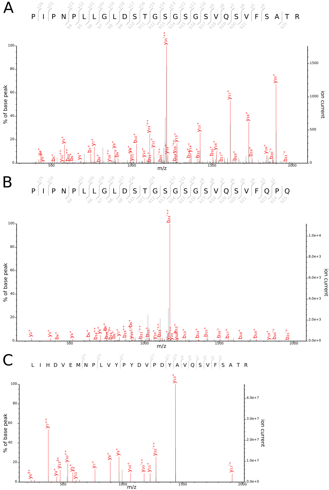
Supplementary Figure S1. Mass spectrometric analysis of tagged products. (A) Fragmentation spectrum of the shift-site peptide derived from V5-tagged 2A-2B*. (B) Fragmentation spectrum of a peptide consistent with 3C-Pro cleavage of tagged 2A-2B at the conserved Q|G encoded just downstream of the frameshift site. (C) Fragmentation spectrum of the shift-site peptide derived from HA-tagged 2A-2B*.
