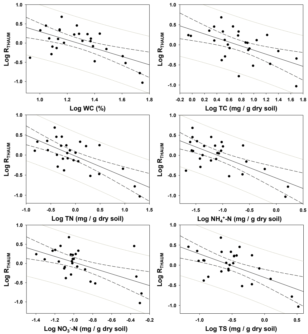
S2 Fig. Significant ( p < 0.05 , ANOVA) regression curves indicating the effects of WC, TC, TN, \text{NH}_4^+\text{-N} , \text{NO}_3^-\text{-N} , and TS upon R_{\text{THAUM}} .
