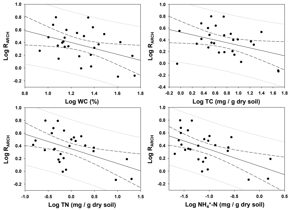
S3 Fig. Significant ( p < 0.05 , ANOVA) regression curves indicating the effects of WC, TC, TN, and \text{NH}_4^+\text{-N} upon R_{\text{ARCH}} .
