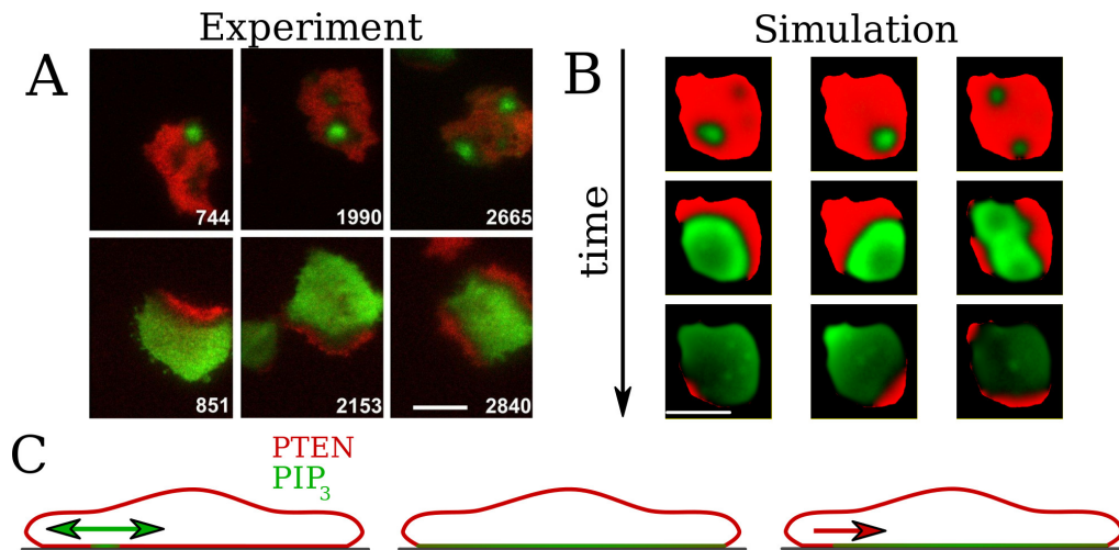
FIG. 4: (A) Merged fluorescent images of PIP 3 (green) and PTEN (red) measured by Gerisch et al. [35], illustrating the coordinated reentry of PTEN. The upper panels show the PIP 3 nucleation spots and the corresponding lower panels represent the PTEN reentry sides at a later time. PTEN always reenters from the location on the cell perimeter which is closest to the PIP 3 nucleation spot. Time is seconds and scale bar represents 10 \mu\text{m} . (B) Snapshots of PTEN reentry (PIP 3 (green) and PTEN (red)) according to our simulations (Bar 10 \mu\text{m} ). (C) Schematic sketch of PTEN/PIP 3 distributions on the membrane postulated in our model and based on experimental results. It illustrates (from left to right) hole formation, PIP 3 wave propagation and coordinated reentry of PTEN. The membrane not attached to the surface continuously exhibits high levels of PTEN even when the surface-attached PTEN membrane level is low and, thus, acts as a reservoir for membrane-bound PTEN.
