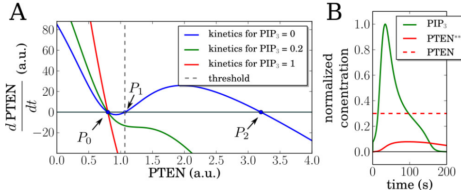
FIG. 3: Dynamics of the proposed model. (A) Local kinetics (neglecting diffusion and noise) of PTEN for different constant PIP 3 values. If the PIP 3 concentration is low (blue curve), PTEN will show bistability corresponding two stable fixed points ( P_0 = 0.8 and P_2 = 3.2 ) and an unstable one ( P_1 = 1.1 ). For higher values of PIP 3 only the lower stable fixed point P_0 remains. Remaining parameter values as in supplementary Table 1. (B) Local normalized concentration profiles (neglecting diffusion and noise) of PIP 3 and PTEN** for constant concentration of PTEN. PTEN* can be calculated from PTEN^* = PTEN - PTEN^{**} . Parameter values in (A) and (B) are given in supplementary Table 1. PIP 3 is normalized to its maximum value while PTEN and PTEN* are normalized by P_0 .
