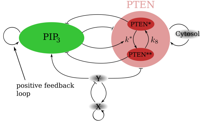
FIG. 2: Schematic representation of the reaction-diffusion model consisting of membrane-bound and diffusible PIP 3 and PTEN. PTEN is assumed to exist in two different forms, PTEN* and PTEN**, with different dephosphorylation rates. Furthermore, PIP 3 and PTEN exhibit a positive feedback loop, resulting in excitable and bistable dynamics, respectively. The substances X and Y prime the formation of holes in the PTEN layer through a stochastic, excitable reaction-diffusion mechanism. Finally, PTEN can detach from the membrane in a PIP 3 -dependent fashion and can quickly re-attach from a constant cytosolic PTEN pool using a positive feedback loop, which is activated by PTEN diffusing back from the non-attached membrane.
