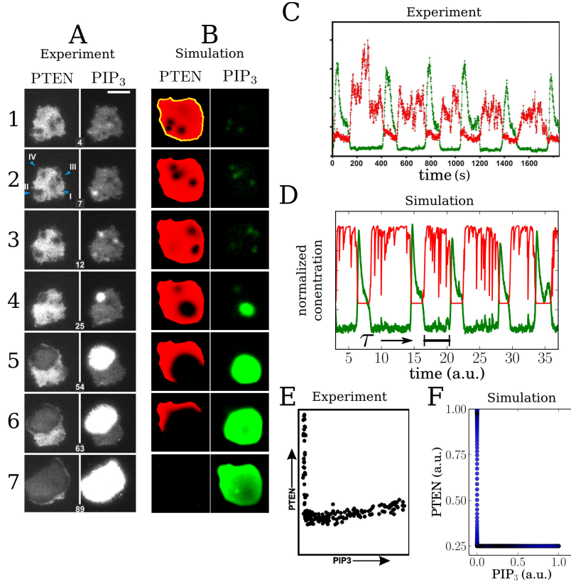
FIG. 1: Comparison of experimental results obtained by Gerisch et al. [35] (A, C, and E) and captured by our simulations (B, D, and F). (A) Polarization in Dictyostelium discoideum cells labeled with PTEN and PIP 3 fluorescent markers and measured using TIRF microscopy. An incomplete polarization cycle is shown (without PTEN reentry). The first three panels from top to bottom for each marker exhibit transient hole formations of PTEN with transient clustering of PIP 3 . The 4th row shows the nucleation of a PIP 3 wave inside a PTEN hole. The remaining panels show the propagation of the PIP 3 and PTEN wave. Time (in minutes) is indicated by the number in each panel set. (B) Simulated polarization cycle of PIP 3 (green) and PTEN (red) following the model presented in this paper and using the parameter values of supplementary Table 1. The cell morphology is indicated by the yellow dashed line and was taken from an experiment. (C) Local time traces of the normalized PTEN (red) and PIP 3 (green) concentration as observed in the experiments [35]. These traces were computed by averaging a 3x3 pixel array at an arbitrary position on the membrane. (D) Corresponding local time traces as determined in our simulations with PTEN in red and PIP 3 in green. The quantity \tau represents the average minimum time delay between the return of PIP 3 to basal levels and a novel excitation. (E) Experimental trajectory of the fluorescence intensity in the PIP 3 /PTEN phase plane obtained at the location of a hole. (F) Corresponding phase trajectory obtained in our simulation.
