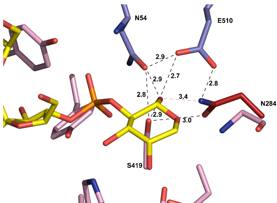
S2a Fig Stick representation of AccA residues interacting with arabinose O1H group in agrocinopine A (in yellow). Residues from the lobe 1, lobe 2 and hinge region are shown in slate, pink and red, respectively.
