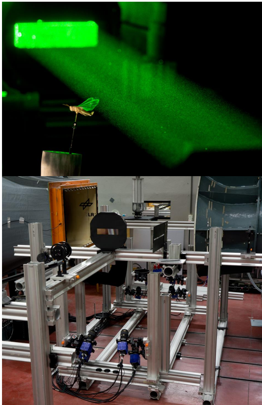
Top panel: The locust in flight on the tether in front of the illuminated volume. Lower panel: The PIV apparatus. In this photograph the calibration plate is lowered into the measurement volume. Photos: Daniel Schantz
