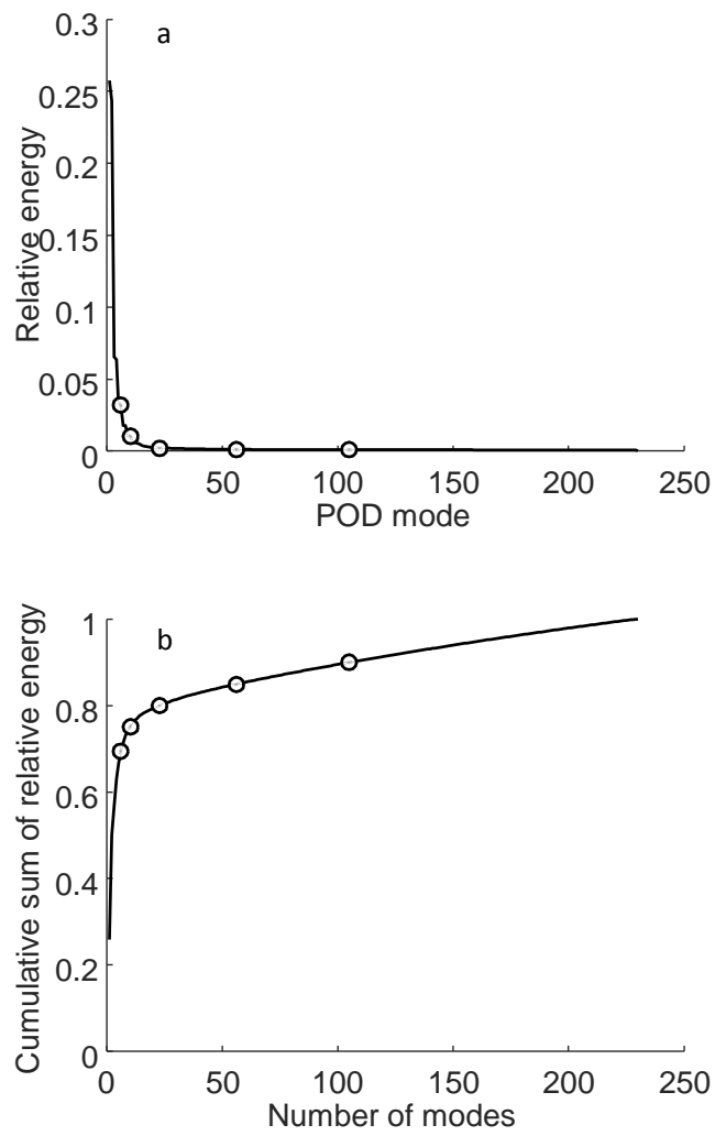
Relative energy distribution in POD modes. The mode number (5, 10, 23, 56 and 105) used for the comparison of consistencies in figure 5 are shown by circles. a) Relative energy in each POD mode scaled so as to sum to 1. b) Cumulative sum of the relative energy in POD mode.
