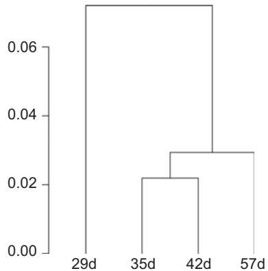
H3K4me3 gene coverage
