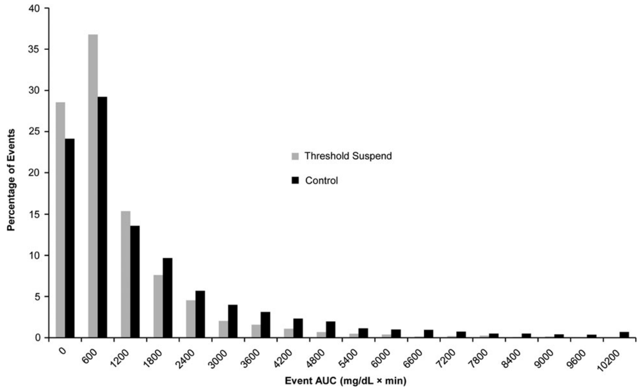
SUPPLEMENTARY FIG. S2. Distribution of area under the curve (AUC) values in the ASPIRE In-Home Study for AUC \leq 65 mg/dL for hypoglycemic events in the Threshold Suspend Group (gray columns) and the Control Group (black columns). Compared with the Control Group, the distribution of events in the Threshold Suspend Group was shifted to the left, indicating a higher prevalence of events with low AUC values.
