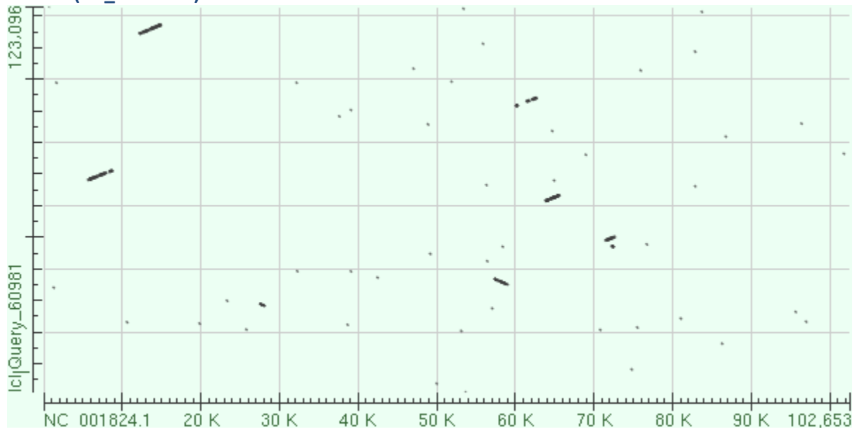
LCDV-1 (NC_001824.1)-SDDV
