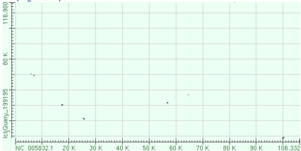
ATV (NC_005832.1)-SDDV
