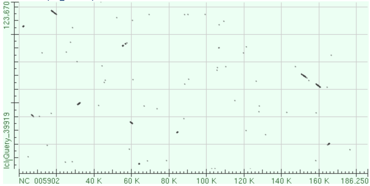
LCDV china (NC_005902)-SDDV
