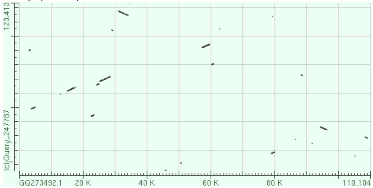
TRBIV (GQ273492.1)-SDDV
