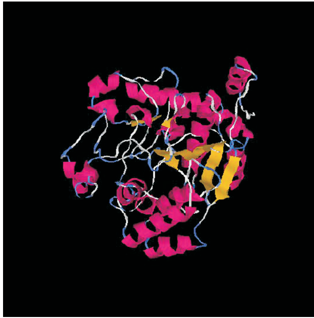
Figure S1 - The predicted 3D structure of CcGolSI generated by the I-TASSER server (Roy et al. , 2010), using 1II0B as a template.
