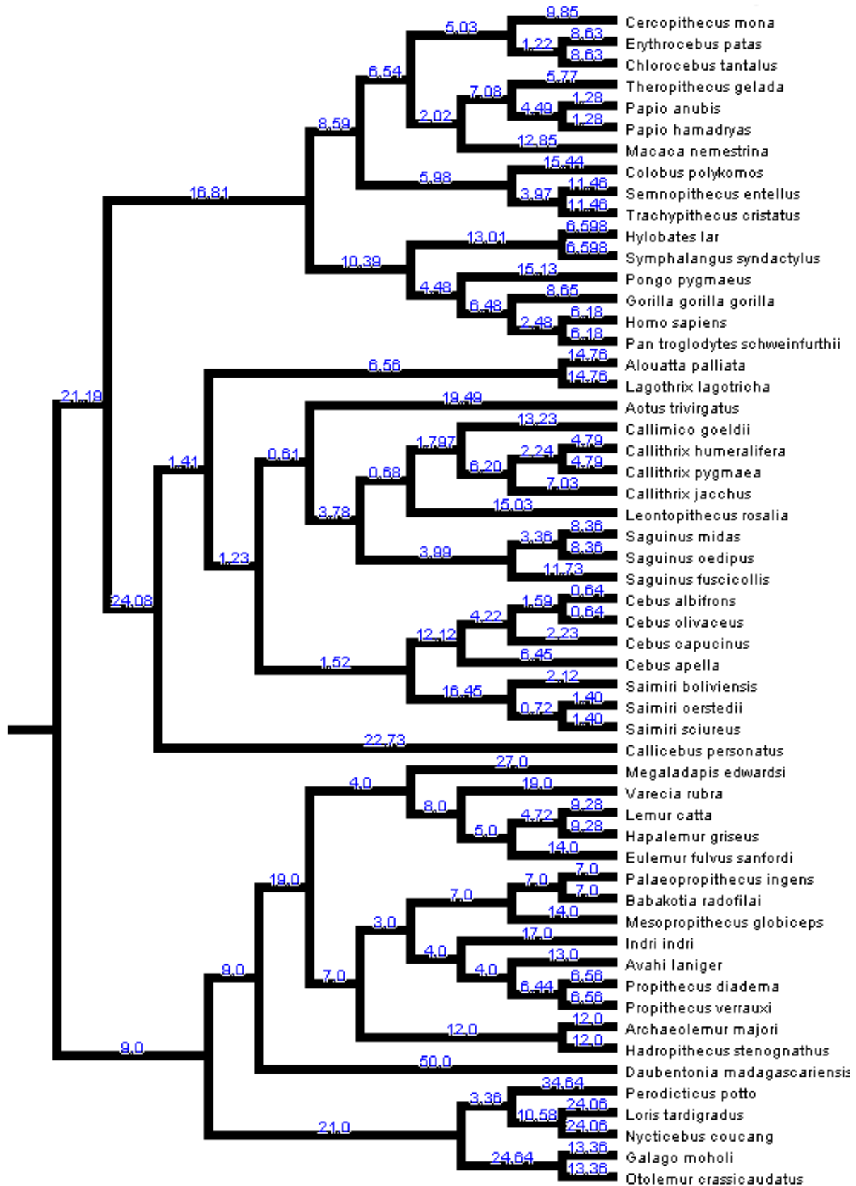
Figure S1. Phylogeny used in PGLS analyses. Includes all extant primates in the study and subfossil lemurs. See the main paper for details & references. To incorporate subfossil lemurs, branch lengths are calibrated as a chronogram. Anthropoid/strepsirrhine divergence date calibrated following Kistler et al. [40]
