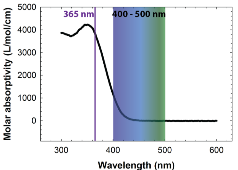
Fig. S3. Molar absorptivity of the photolabile moiety on the photodegradable macromer. The nitrobenzyl ether based photolabile moiety absorbs 365 nm UV light strongly compared to 400 to 500 nm visible light wavelengths.
