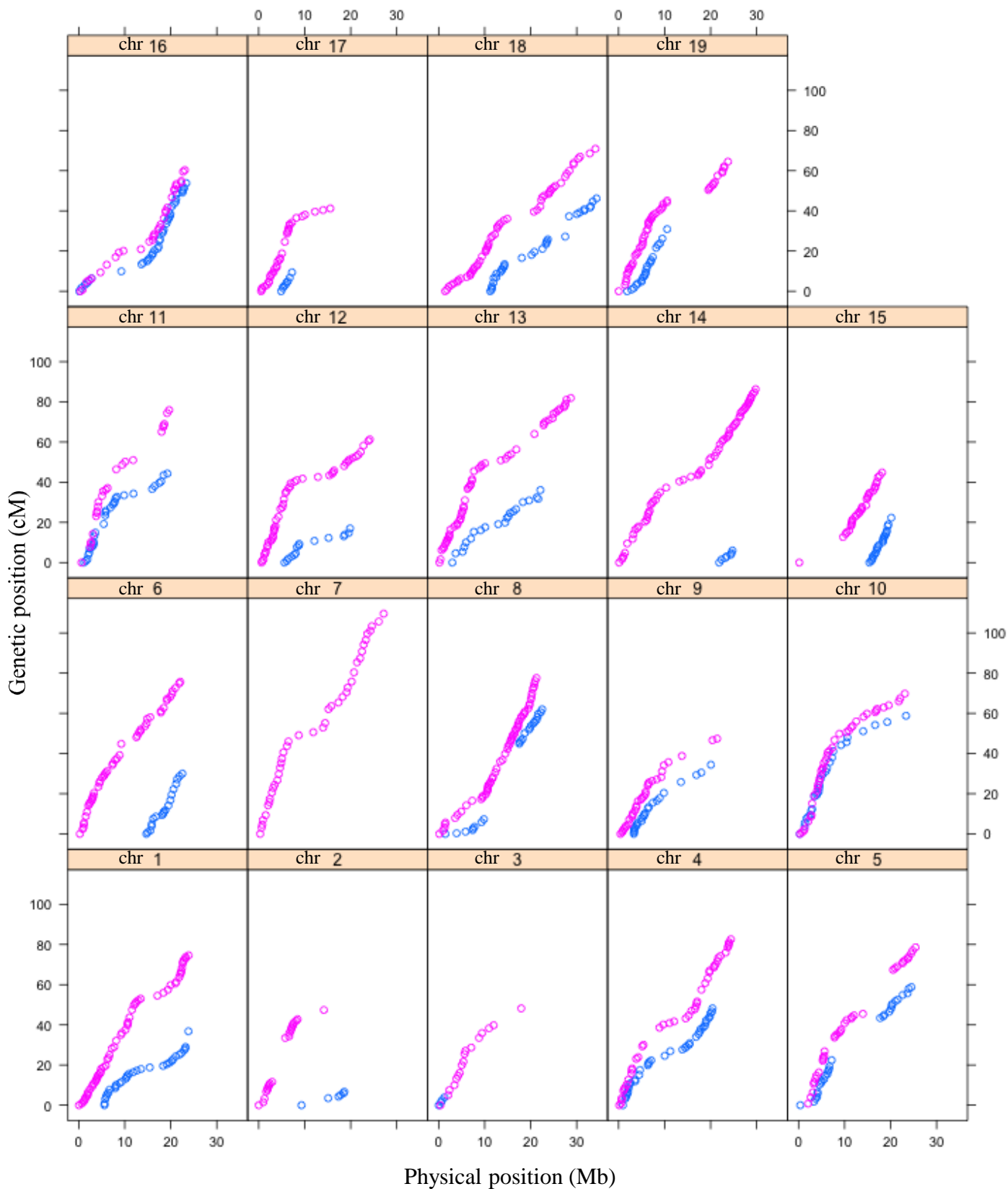
Figure S4. SNP positions on genetic maps as a function of their physical position on the reference genome version 12X.2. The maternal parent is the Picovine (blue circles) and the paternal parent is the Ugni Blanc flb (pink circles).
