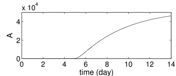
(A) q = 10^{-7}
