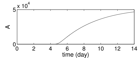
(A) q = 10^{-7}
