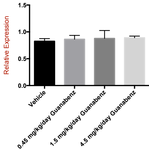
Relative Atf4
