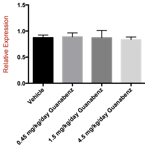
Relative Chop
