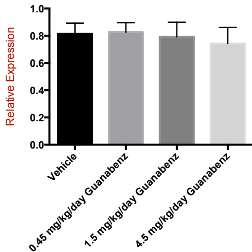
Relative Bcl2
