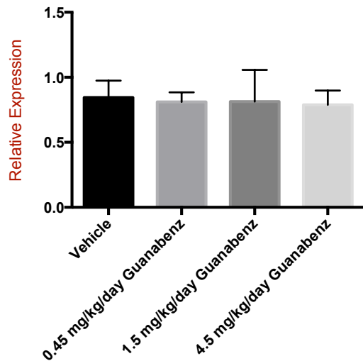
Relative Ccnd1
