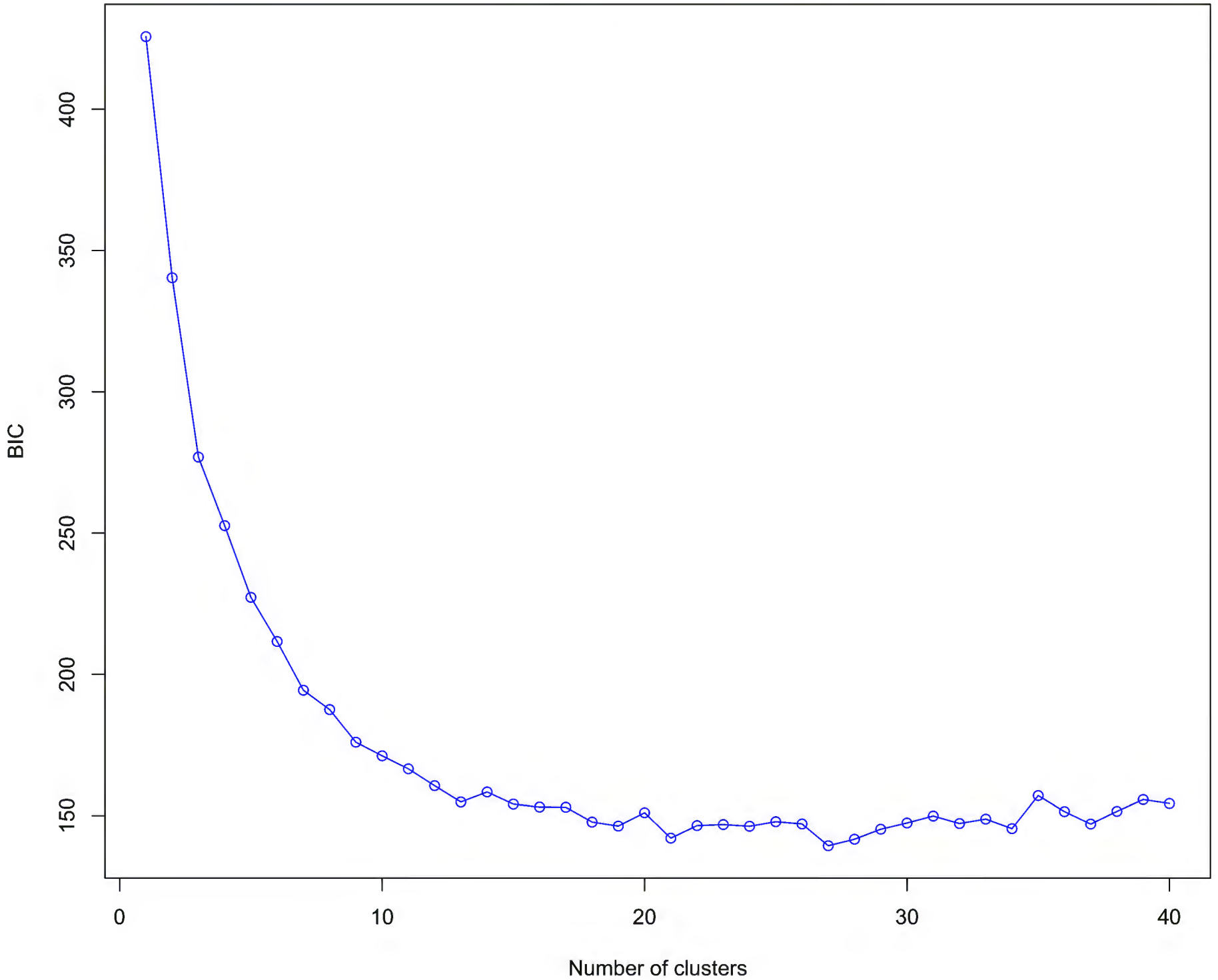
Value of BIC versus number of clusters
