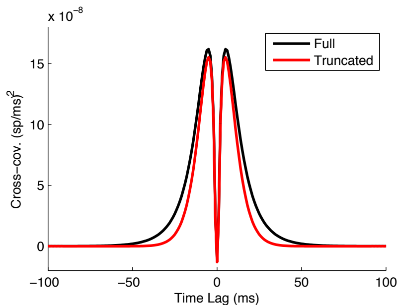
Figure 1. Truncated vs full spike train cross-covariance functions. Black, average spike train cross-covariance function of the network of Fig. 2. Red, truncated approximation (Eq. 7 of main text) of the average spike train cross-covariance function. When integrated against the balanced, depression dominated STDP rule, the full theory is 1.06 times as large as the truncated.
