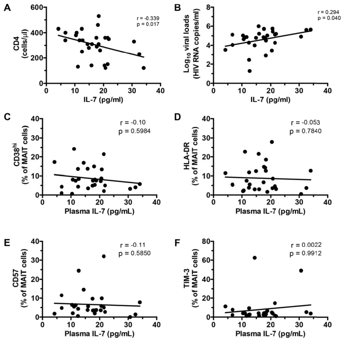
S6 Fig. Plasma IL-7 levels weakly correlate with CD4 counts and plasma viral load, but not with MAIT cell activation markers. Relationships between plasma IL-7 levels and CD4 counts (A), plasma viral loads (B), as well as with the MAIT cell activation markers CD38 (C), HLA-DR (D), CD57 (E), and TIM-3 (F) was assessed using Spearman's rank correlation in 31 ART-untreated HIV-infected patients.
