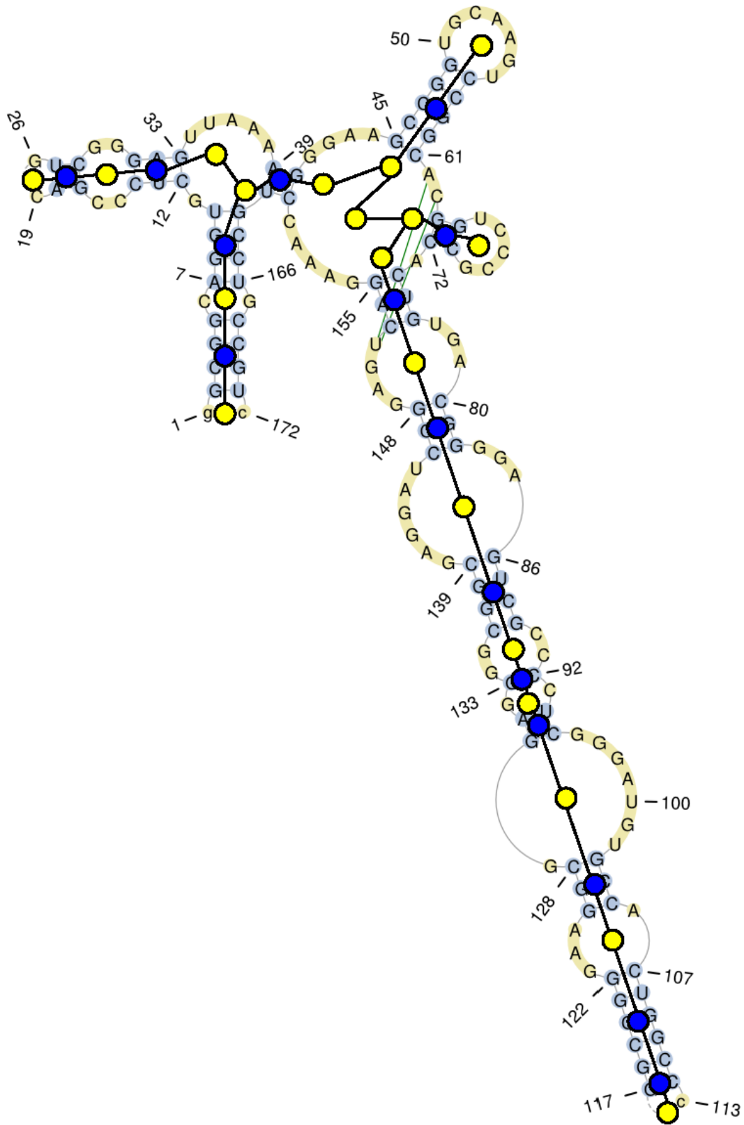
Figure S2: Model for a four-way junction. Simple modeling of a four-way junction. Five players are used to model the four-way junction. They are located as if the junction consisted of two three-way junctions and a linker.
