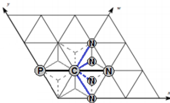
Figure S6: Strategies on the lattice. The current player, C, has to choose the direction of the next player, N, according to the direction of the previous player, P. If player C is frozen, this player can only choose the strategy corresponding to the black line; if not frozen, this player can choose to follow any of the blue lines.
