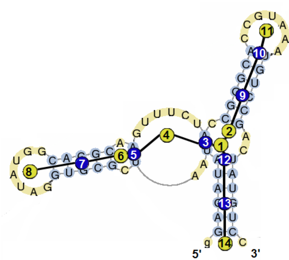
Figure S8: Ordering of the players for the game. Players from the largest junction play first, and the other players are numbered according to a depth first search, starting from the first largest junction according to 5'-3' ordering.
