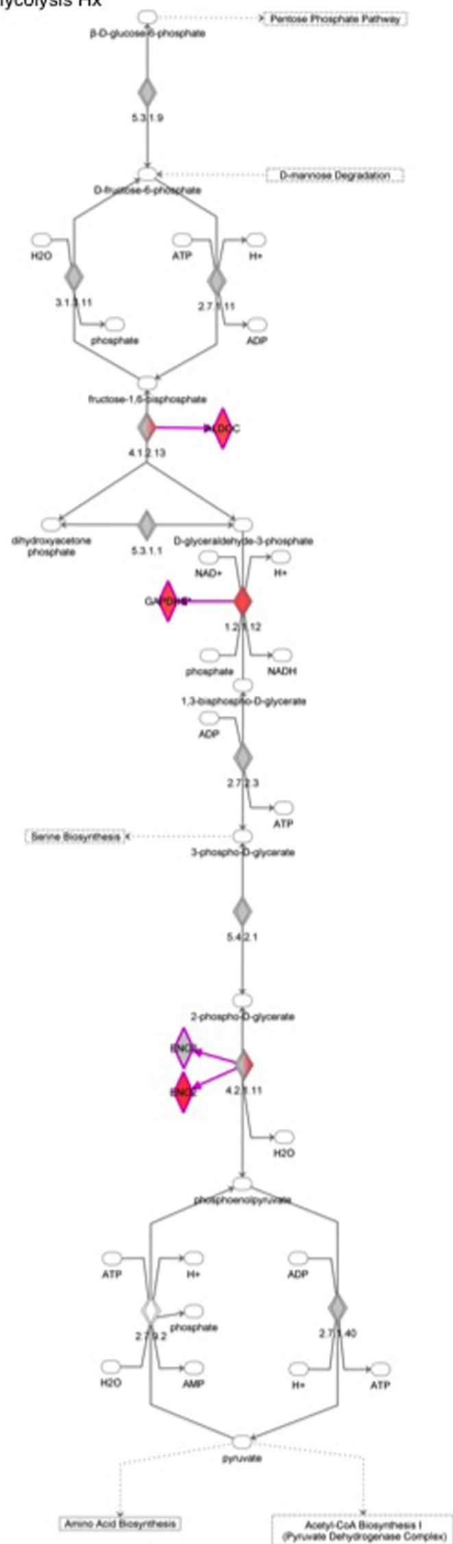
Supplemental Figure S6. Changes in metabolic pathways in Vdac1 -/- vs Wt MEF. (A and B) Ingenuity Pathway Analysis of the metabolic activity of Vdac1 -/- vs Wt MEF in (A) normoxia and (B) hypoxia. Red color code for up-regulation
