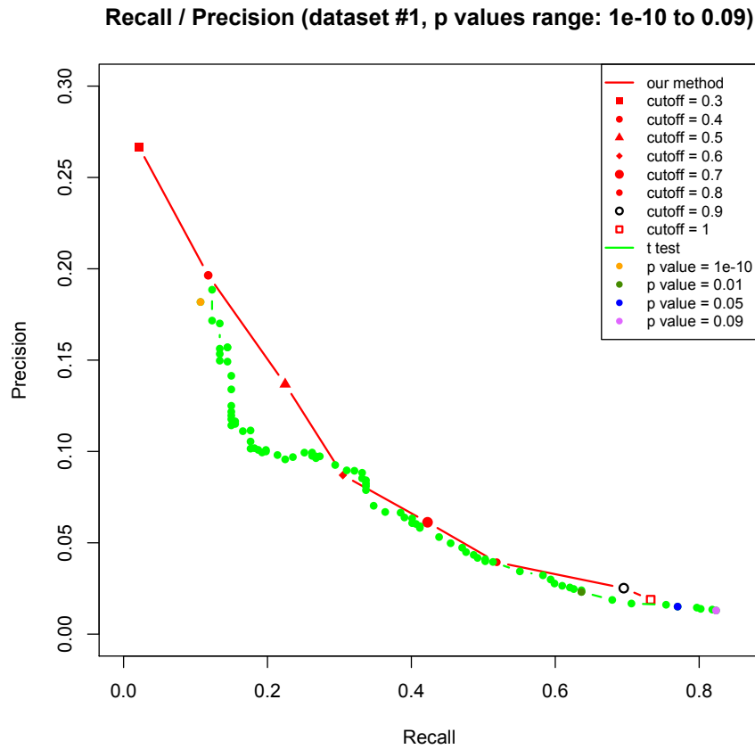
Figure 1: Comparison of Precision/Recall for the complete set of genes selected by our tool and t -test as potential markers for the examined tissues using data set #1.
