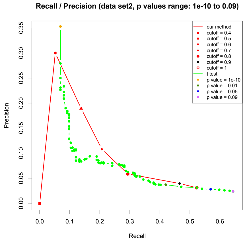
Figure 2: Comparison of Precision/Recall for the complete set of genes selected by our tool and t -test as potential markers for the examined tissues using data set #2.
