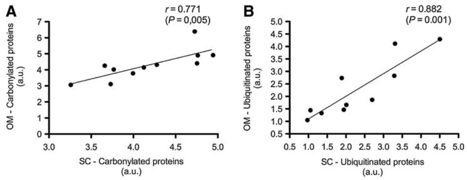
SUPPLEMENTARY FIG. S3. Correlation of carbonylated and ubiquitinated proteins between human SC and OM adipocytes. (A) Levels of carbonylated and (B) ubiquitinated proteins positively correlate between paired SC and OM adipocytes. Pearson's correlation ( r ) and p -value are indicated for each graph.
