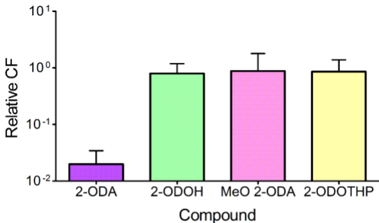
Figure S1. COIN activity of 2-ODA analogs. Conjugation frequency (CF) represented in logarithmic scale in the presence of 2-ODA and derivatives at 1 mM, relative to a control without added compounds ( 10^0 ). Values represent the mean + SD of at least three independent experiments measured by HTC assay.
