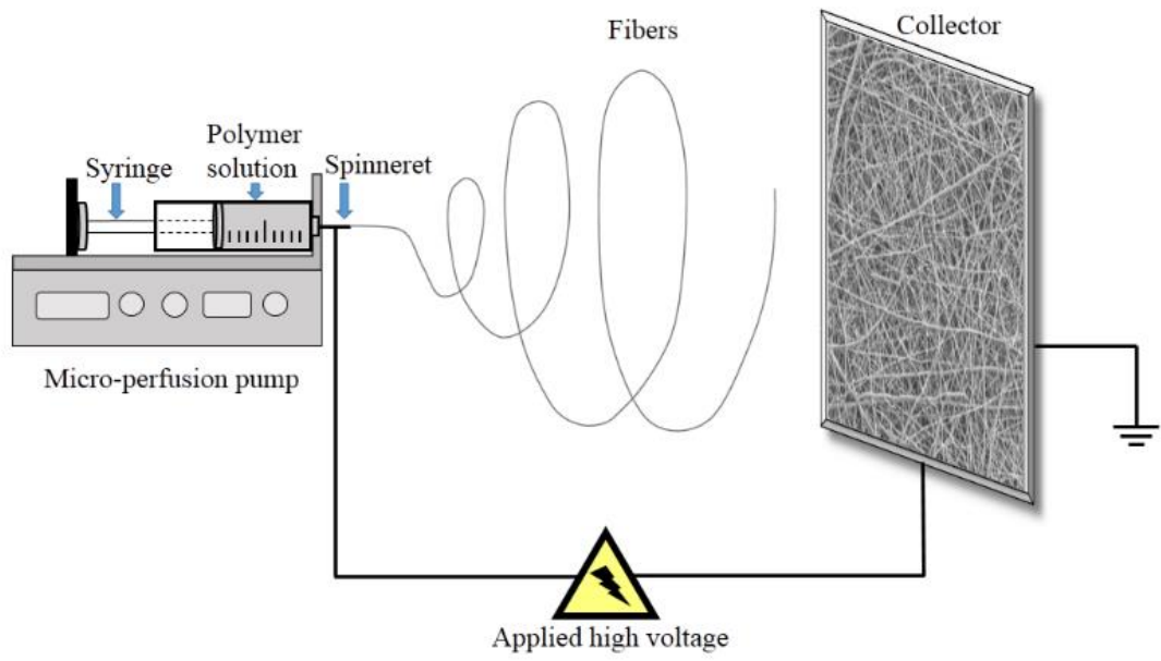
Figure S1. Schematic diagram of a typical horizontal electrospinning system.
