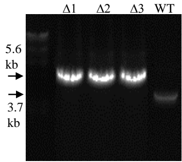
FGSG_14031
