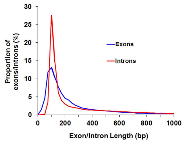
S1 Figure: Exon and intron sizes in the wheat genome. Exon and intron sizes were calculated from the GFF annotation file supplied with v21 of the IWGSC wheat genomic survey sequence at Ensemble Plants .
