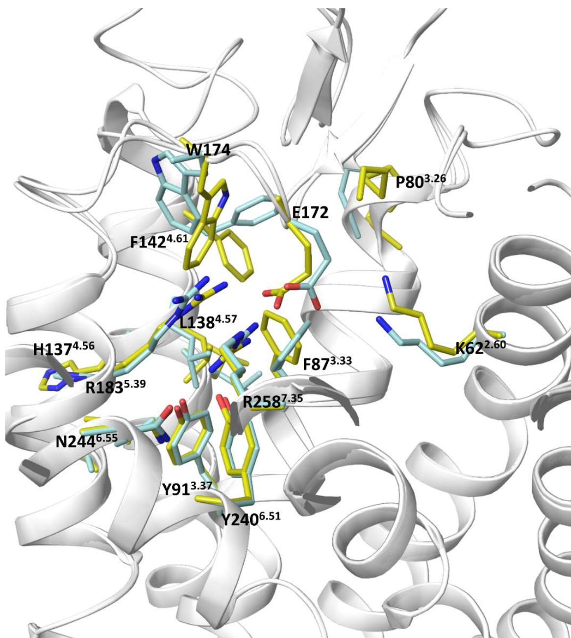
Additional Figure 4S. The superimposition of the FFA1 crystal structure and a characteristic conformation of FFA1 from conformational search of the FFA1 crystal structure without the ligand. The figure shows changes in the conformation of F87 3.33 , F142 4.61 and W174 EL2 , which close the interhelical space between helices 3 and 4.
